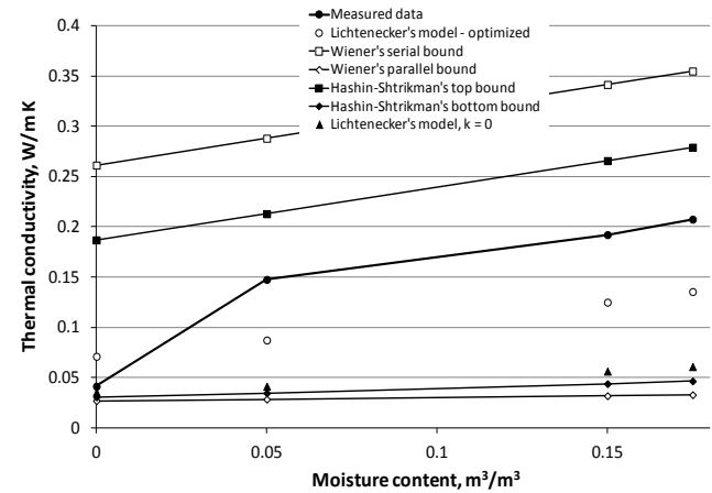
Fig. 4. The thermal conductivity dependence on MC (1 st part of the curve)
