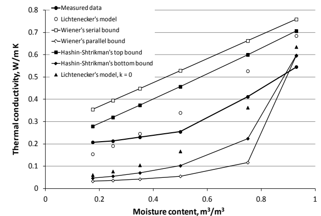
Fig. 5. The thermal conductivity dependence on MC (2 nd part of the curve)
