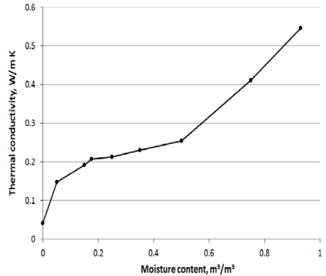
Fig. 3. Thermal Conductivity of HMW as a function of MC
