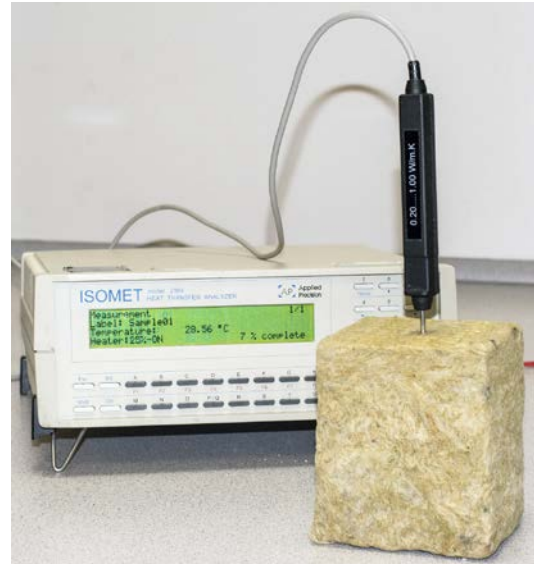
Fig. 2. Isomet 2104 and needle probe during test of a HMW sample
