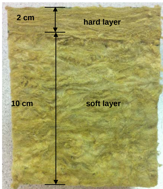
Fig. 1. Studied HMW board
